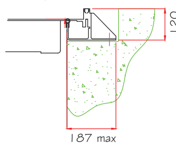
TYPICAL FIXING
